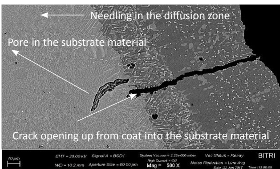
Fig. 4. Sectioned tip
