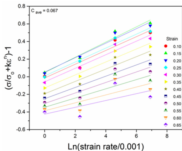
Fig. 4. Plot of \frac{\sigma}{\sigma_0 + K\varepsilon^n} vs. \ln \dot{\varepsilon} at reference condition.
