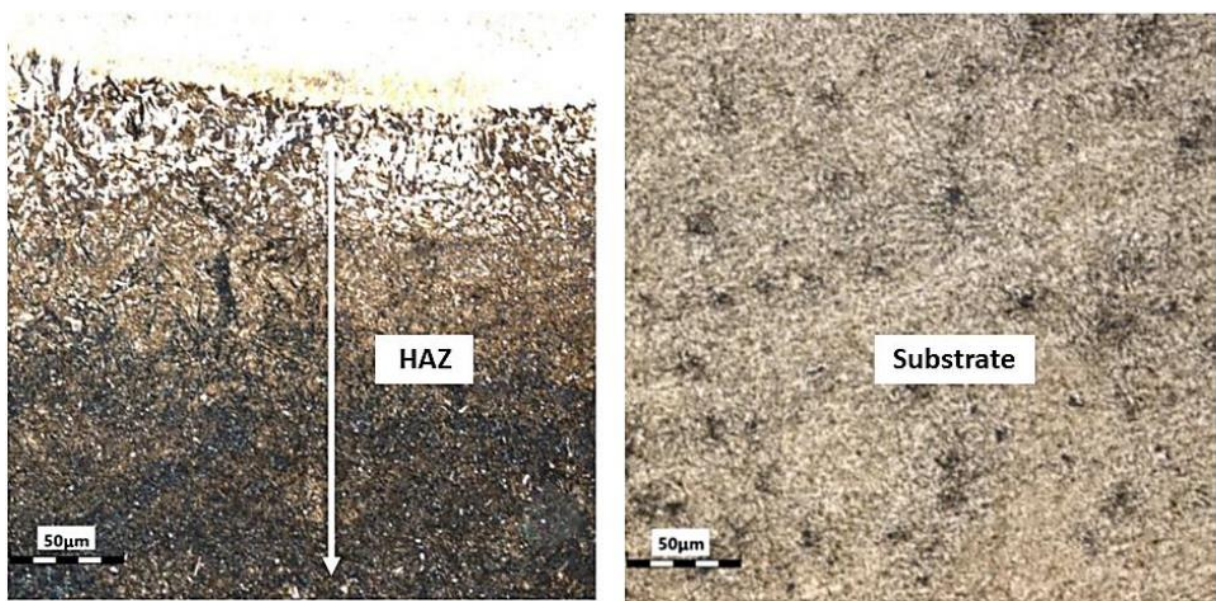
(a) ..... (b) Fig. 10. Detail of the HAZ (a) and substrate (b) AISI H13.
