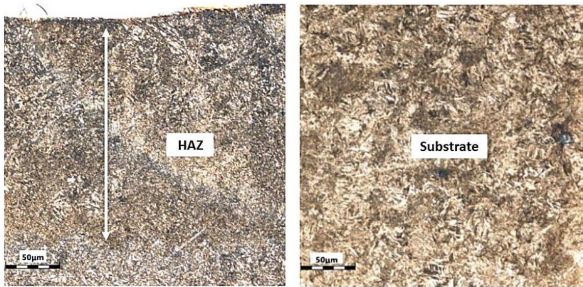
(a) ..... (b) Fig. 9. Detail of the HAZ (a) and substrate (b) AISI 4140.
