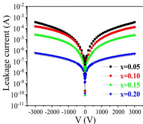
Fig. 13. Plots of Applied voltage (V) and leakage current (I) for (1-y)Bi_{1-x}Nd_xFeO_{3-y}PbTiO_3 solid solutions with y= 0.1 and varying x compositions
