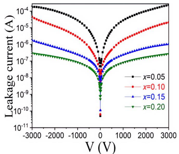
Fig. 14. Plots of Applied voltage (V) and leakage current (I) for (1-y)Bi_{1-x}Nd_xFeO_{3-y}PbTiO_3 solid solutions with y= 0.2 and varying x compositions
