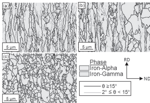
Fig. 3. (a)-(c) Grain boundary and phase maps of the specimens ARB processed by 6-cycle and annealed at 773, 823 and 873 K respectively.
