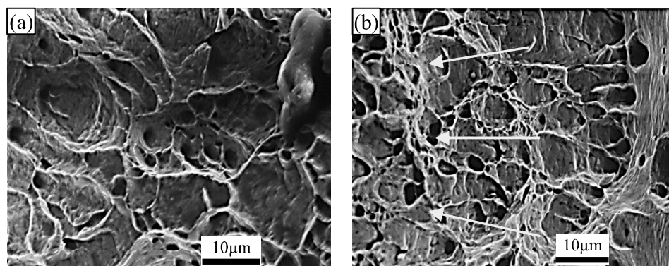
Fig. 7. SEM images of fractured surfaces after the tensile tests of a) unprocessed state, b) after seven cycles of CFS.
